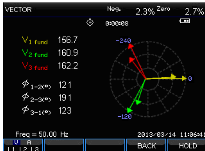
Picture: Vector diagram for correctly connected Analyzer
