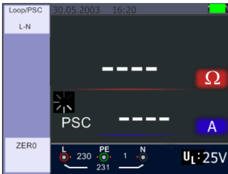
L-N Line Impedance – When measuring
