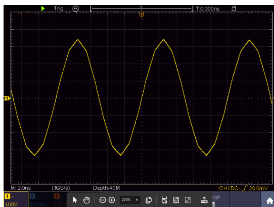
Figure 4.2 x Interpolation
