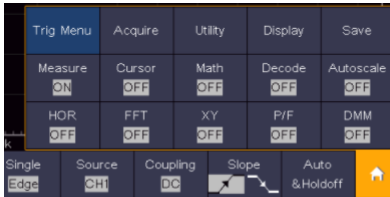
Figure 3.7 Menu principal
