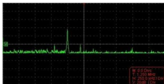
Hanning Fenster
