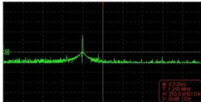
Hamming Fenster
