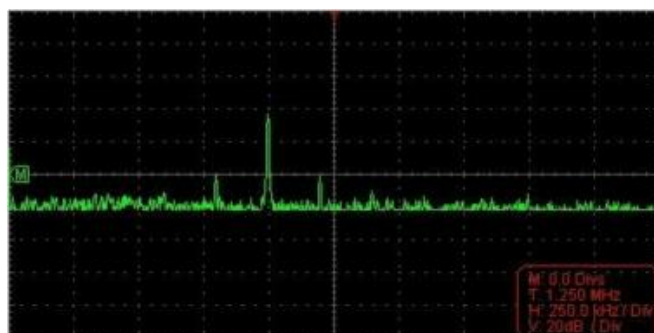
Blackman Fenster
