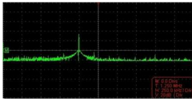
Hamming window
