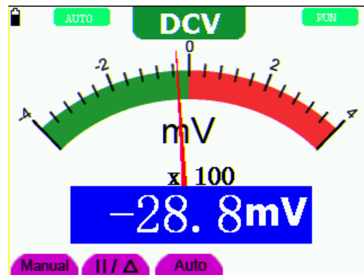
Screenshot Multimeter
