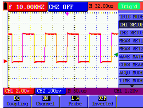
Figure 36: DC Coupling
