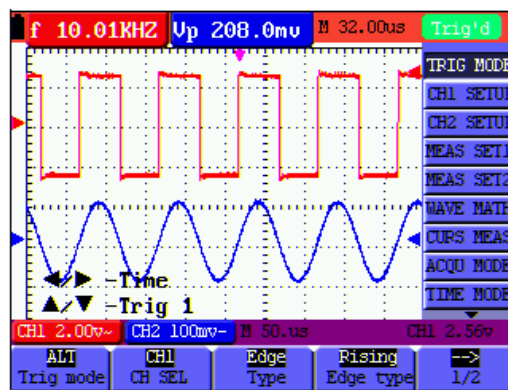
Figure 43: Alternate Trigger
