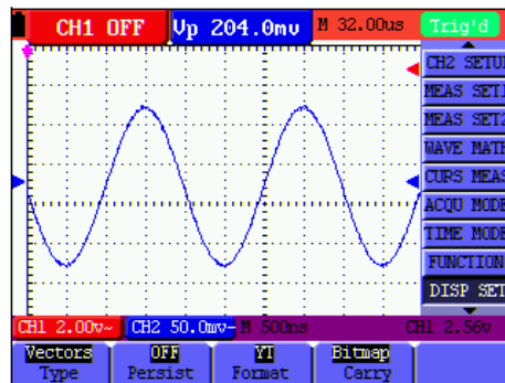
Figure 45: Vector Style
