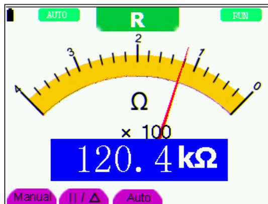
Figure 21: Resistance Measurement
