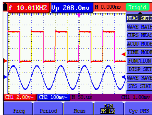
Figure 11: Automatic Scope Measurements
