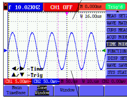
Figure 60: Window Setting
